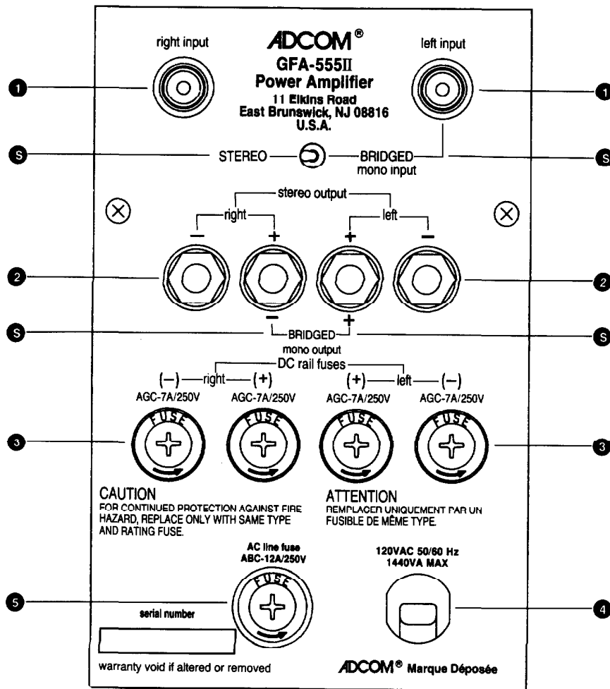
GFA-555II Rear Panel Diagram
